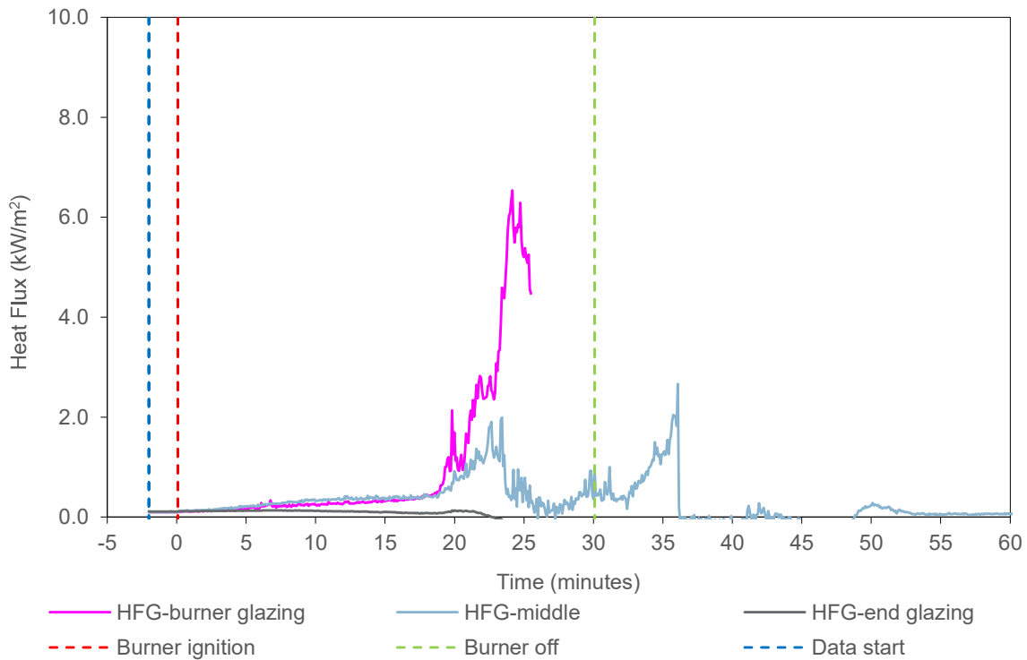
Figure 10 Heat flux data collected by heat flux gauges behind the glazing units 1
