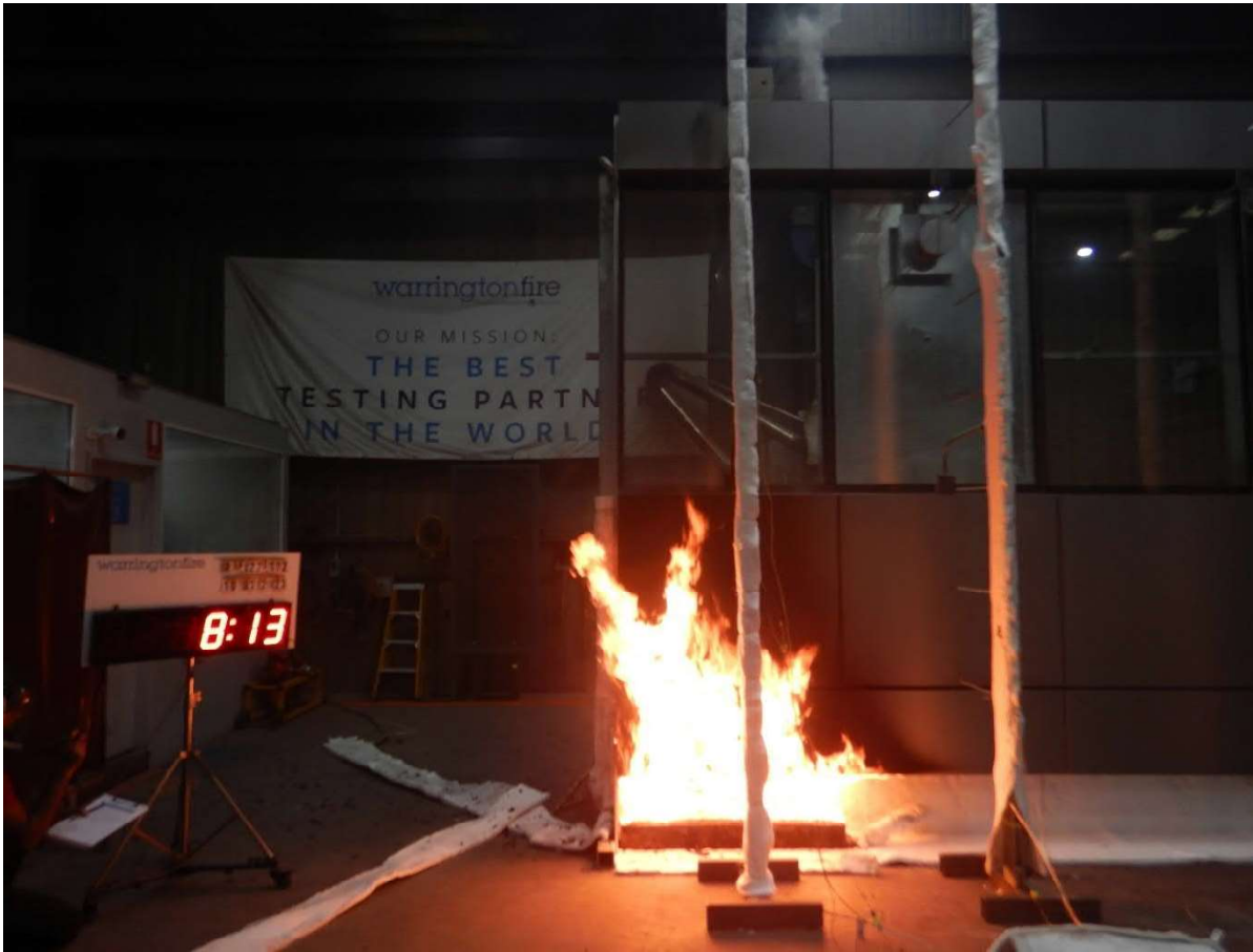
Figure 29 The specimen 8 minutes 13 seconds into the test (burner output at 300 kW)
