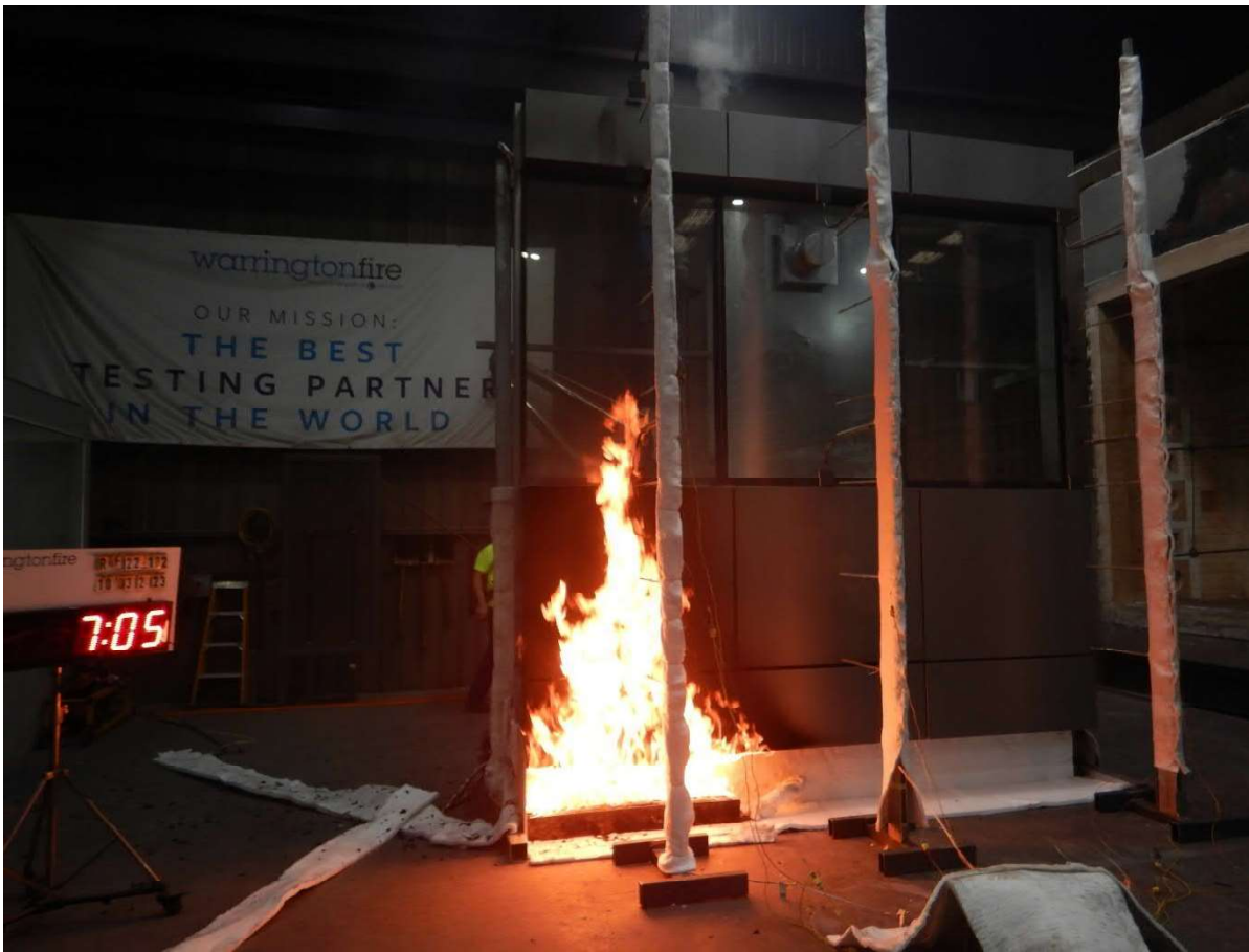
Figure 27 The specimen 7 minutes 5 seconds into the test (burner output at 300 kW)
