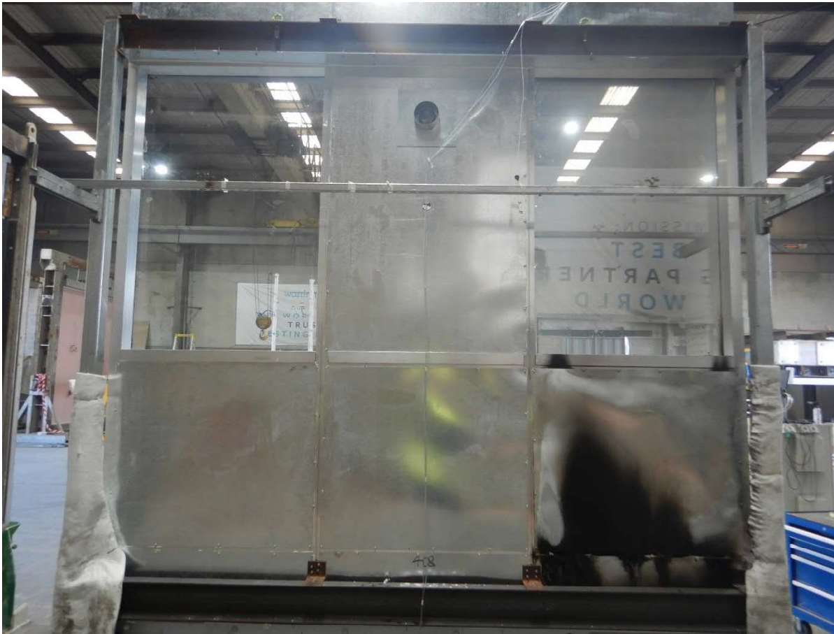
Figure 61 The specimen at end of test – unexposed side.
