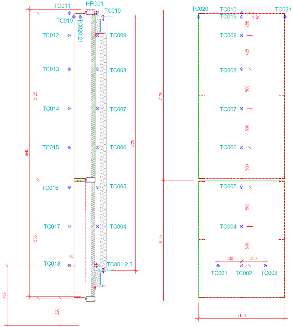
Figure 1 Instrumentation location
