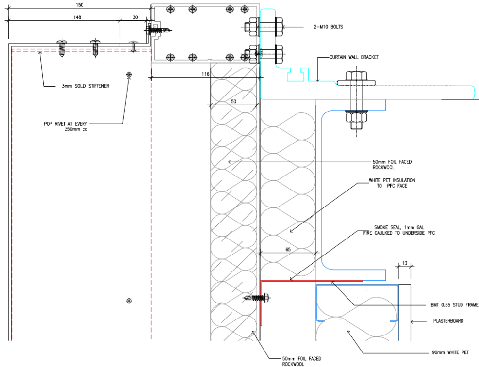
Figure 11 System assembly – top edge detail
